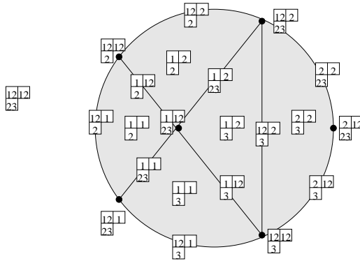
Figure 3. The empty-face tableau and simplicial complex for \lambda = (2, 1) and \vec{n} = (2, 3) .
